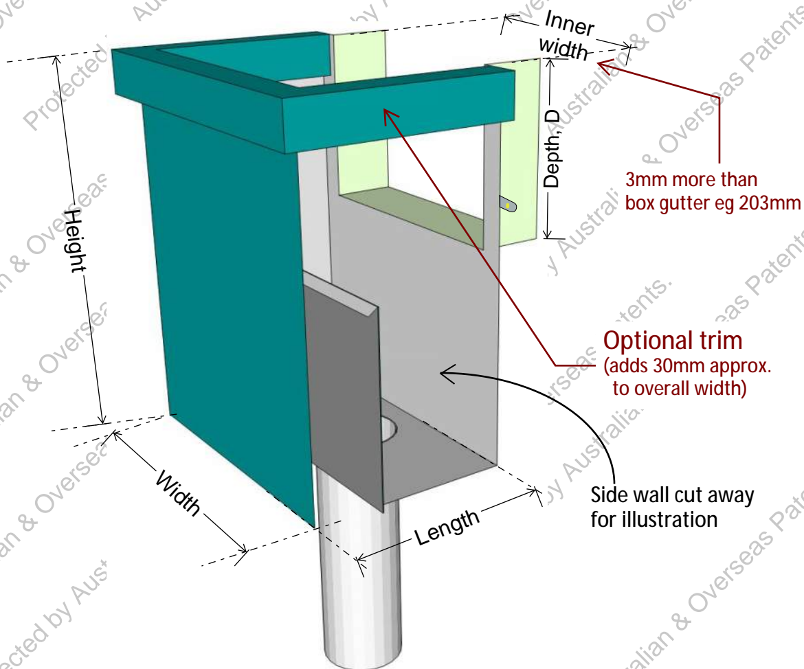
NON-STANDARD RAINHEAD DIMENSIONS for R-200-xxx & R-300-xxx series
